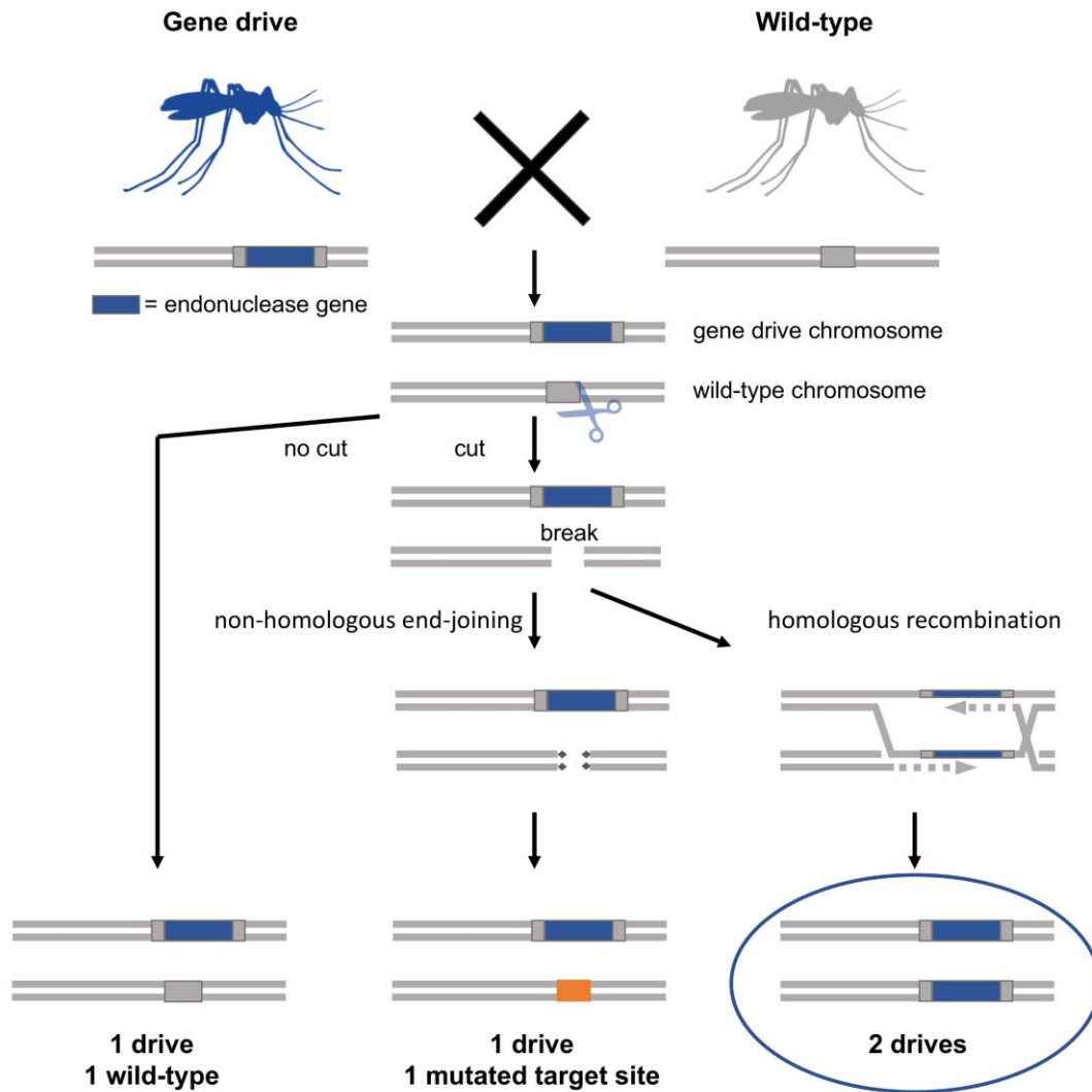
Figure 2 The spread of homing endonuclease gene drives (adapted from Esvelt et al., 2014)
